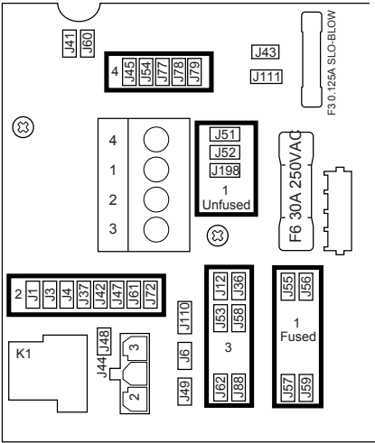
BREAKER TERMINAL CONNECTIONS L1 = All components
