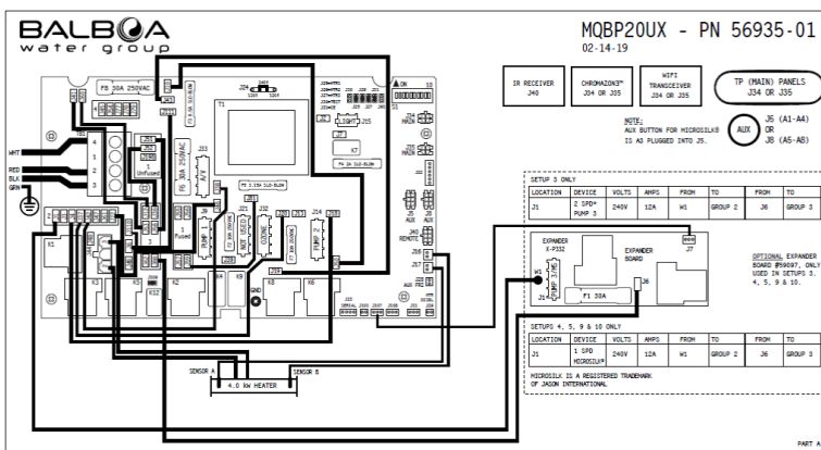
Wiring Diagram
